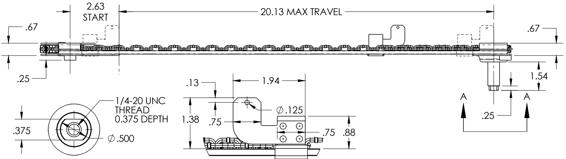
VIEW A-A SCALE 1 : 1
