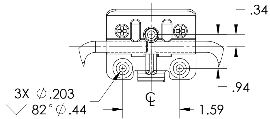
DETAIL A SCALE 1 : 2 (COVER REMOVED)
