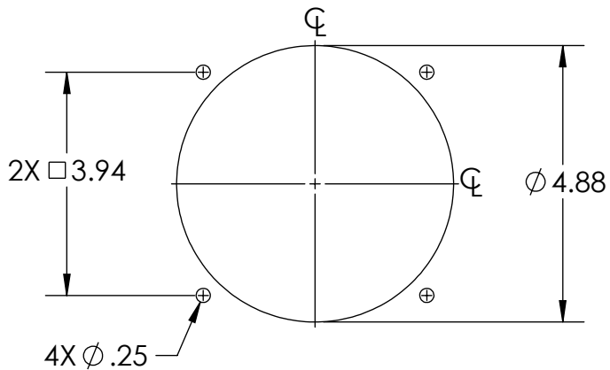
D-RING CUTOUT
