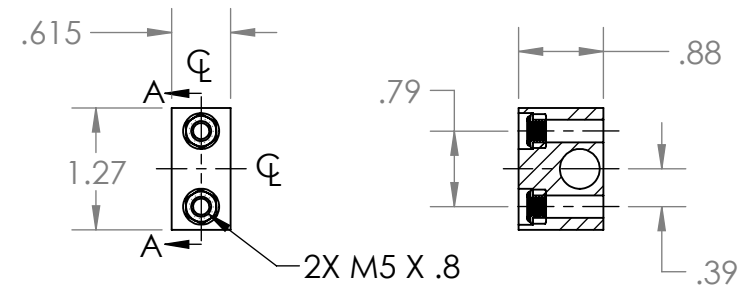
DRAWER BLOCK SCALE 1:2
